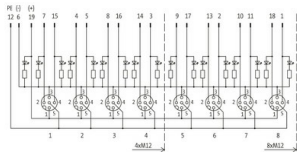
M12-Females 5-pole
