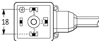
Female
