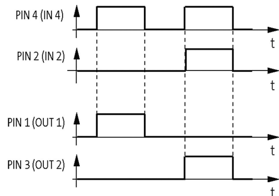
Time diagram
