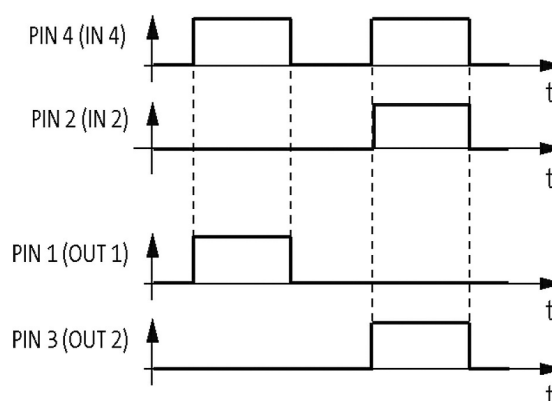
Time diagram
