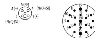
M12-Females 5-pole M23-Plug 19-pole
