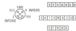
M12 Females 5-pole
