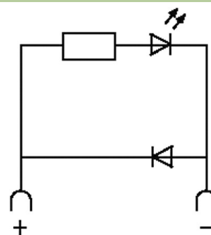
Diode + LED
