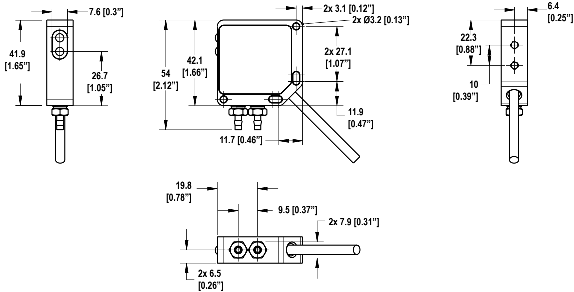
Figure 1. Dimensions
