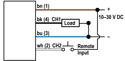
Figure 16. Channel 1 = PNP Output, Channel 2 = PNP Remote Input
