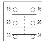
Actuator removed
