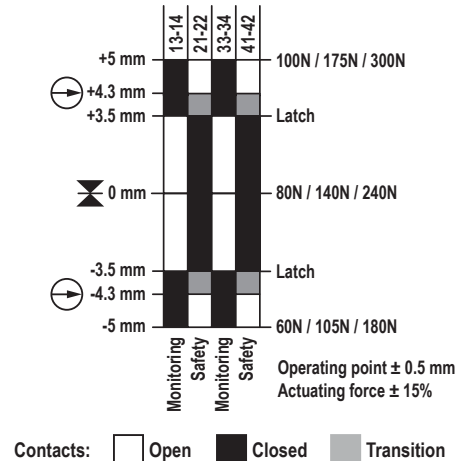
Figure 2. Switching Diagram
