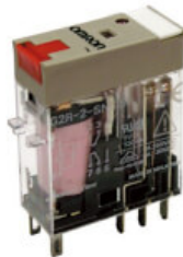
G2R-2-SNI 12VAC (S) Relay, plug-in, 8-pin, DPDT, 5 A, mech & LED indicators, lockable test button, label facility
