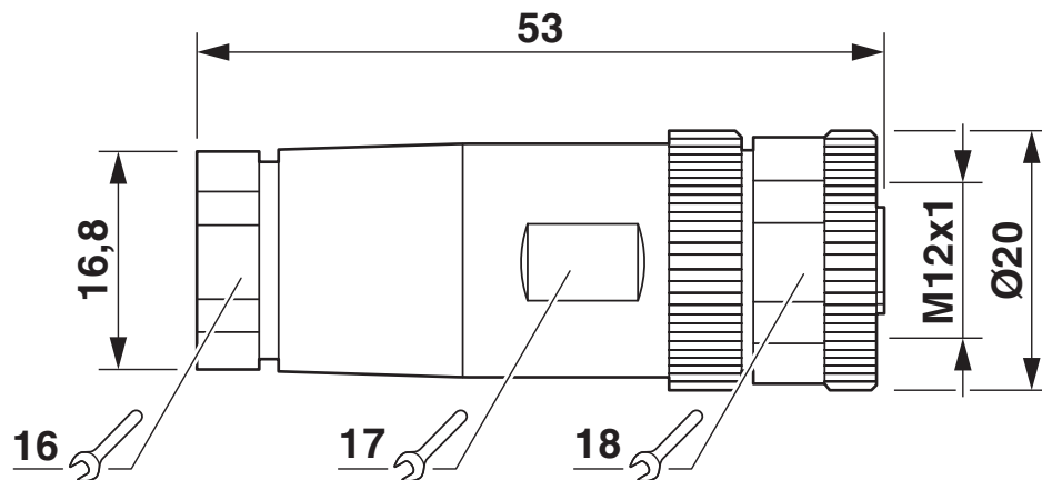
Dimensional drawing
