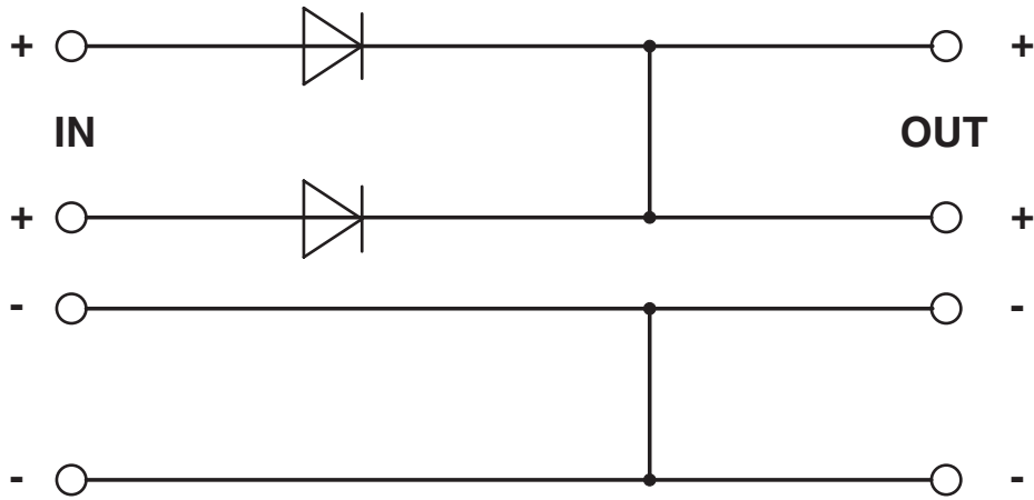
Block diagram
