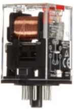
MKS2PI 230VAC Relay, plug-in, 8-pin, DPDT, 10 A, mech indicator, test button
