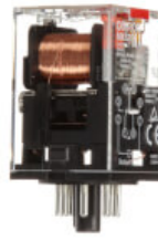
MKS2PI 110VAC Relay, plug-in, 8-pin, DPDT, 10 A, mech indicator, test button
