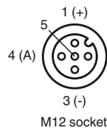
M12 socket
