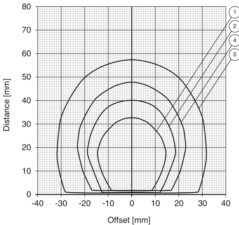
Reading range in air IPC03-20..
