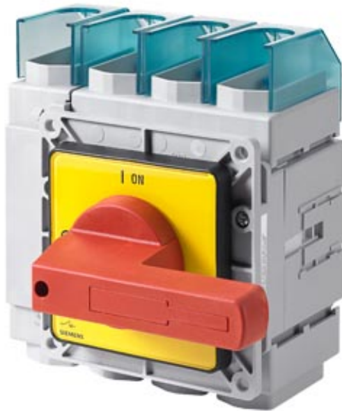
MAIN SWITCH 4-POLE FRONT MOUNTING IU=250A,P/AC-23A AT 400V=132KW ROTARY ACTUATOR RED/YELLOW (EMERG. STOP) FOUR-HOLE MOUNTING
