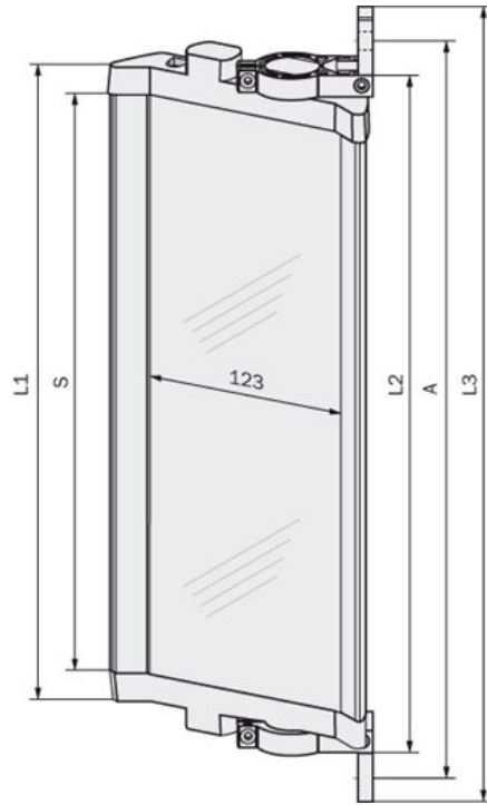
Sliding nut groove for side mounting
