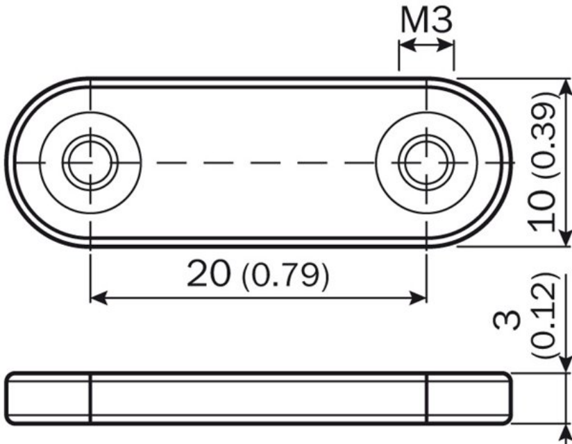
All dimensions in mm (inch)
