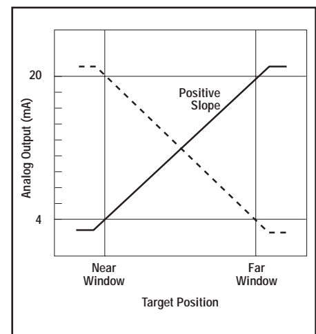
Figure 6. Output current as a function of target position
