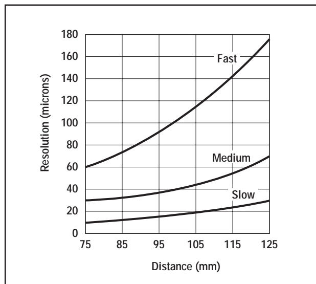
Figure 3. L-GAGE LG10 Series resolution, with respect to speed (typical, using a white ceramic target)
