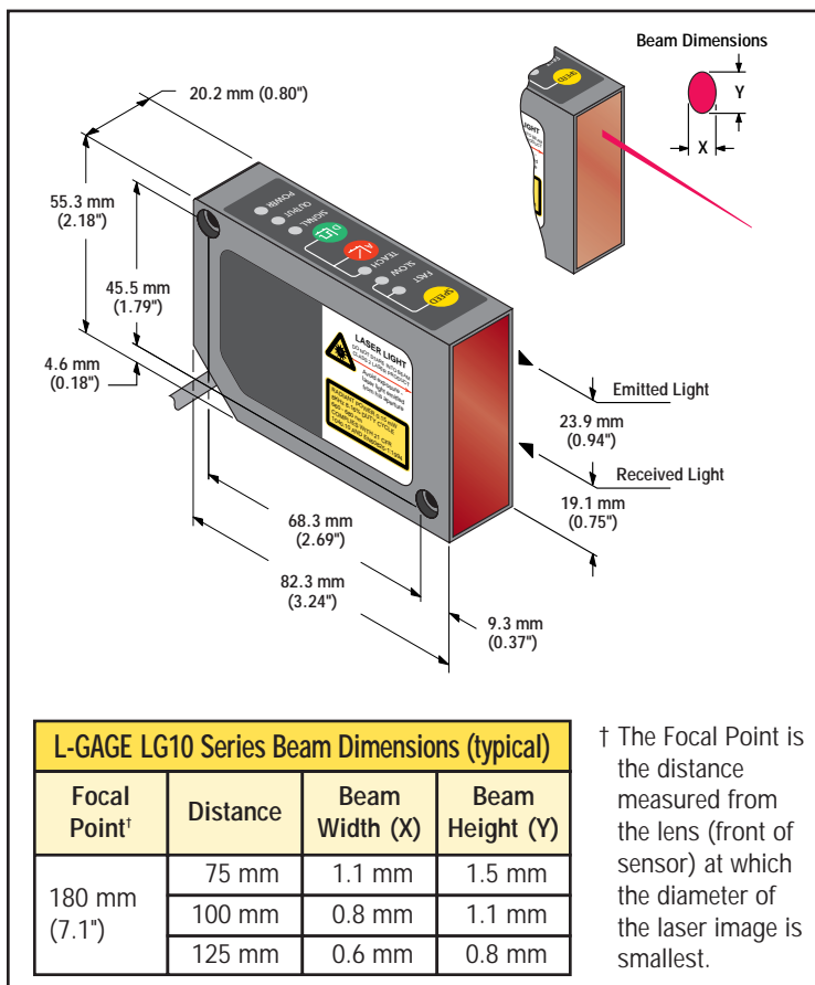
Figure 2. L-GAGE Laser Gauging Sensor and beam dimensions
