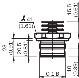
Housing with circular plug-in connector M12 x 1
