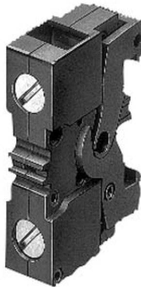
ACTUATOR-/INDICATOR COMPONENT CONTACT BLOCK WITH 1 CONTACT ELEMENT GOLD-PLATED CONTACTS SCREW TERMINAL, 1NO
