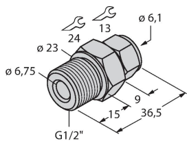
CF-M-6-G1/2-A4 9910530
