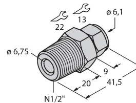
CF-M-6-N1/2-A4 9910529
