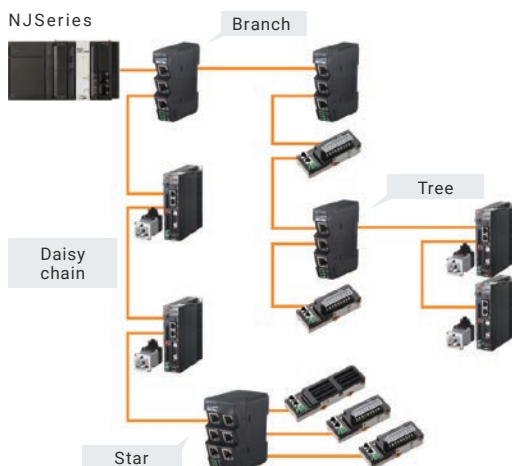
Figure 1. Wiring example
