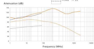
Shielding effectiveness measurements
