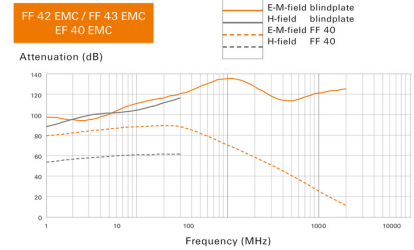
Shielding effectiveness measurements
